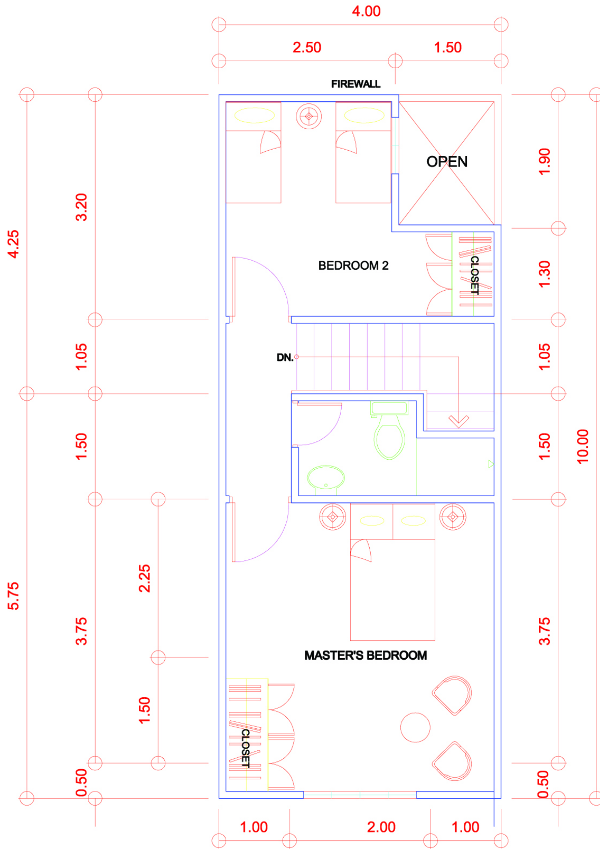
SECOND FLOOR PLAN SCALE 1:50MTS
